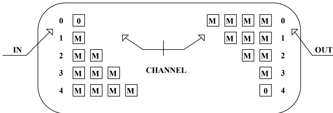
Figure 2-7 Conceptual Diagram of the Convolutional Interleaver and De-leaver
