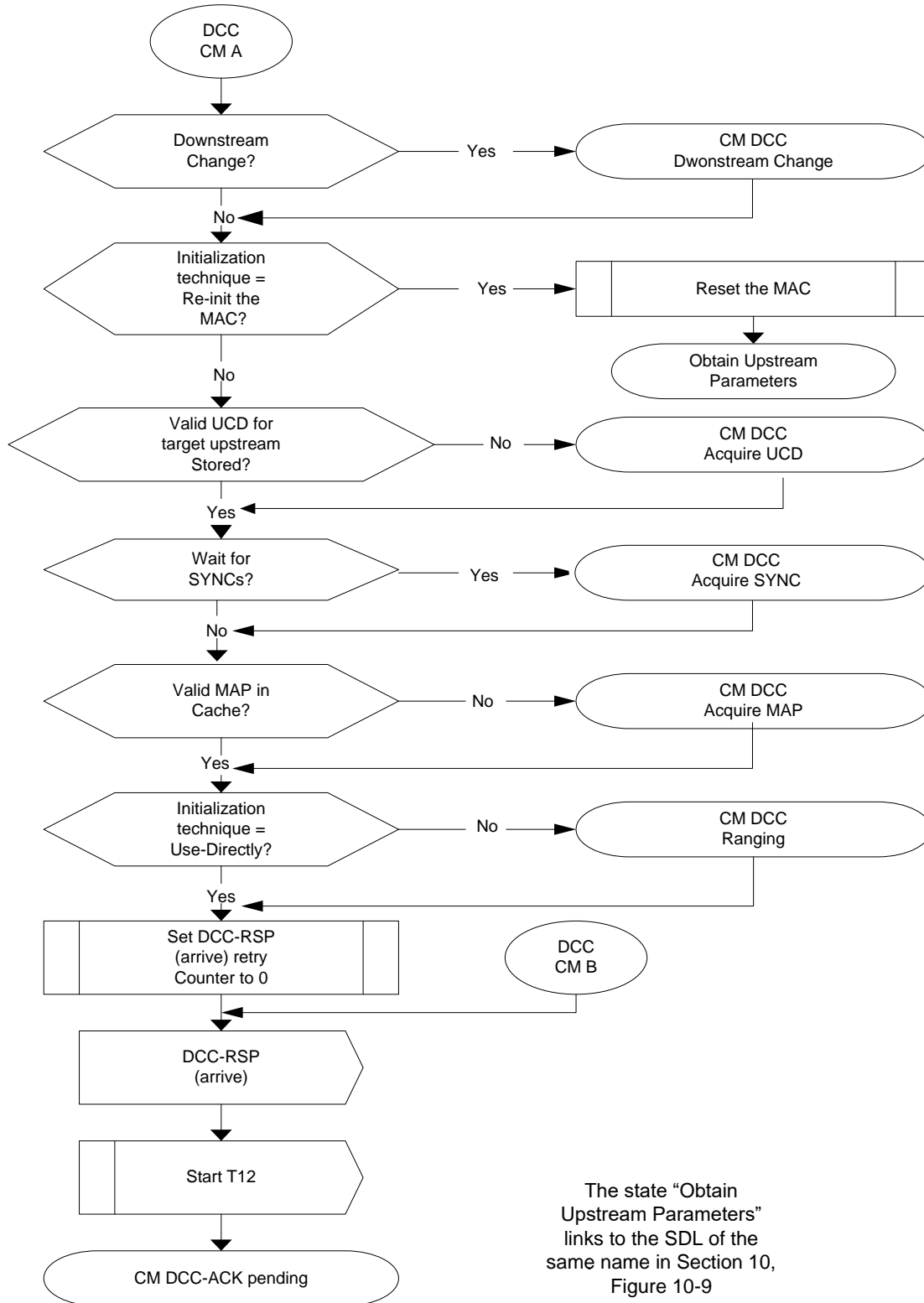
Figure 11-47 - Dynamically Changing Channels: CM View Part 2
