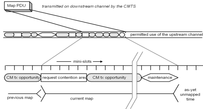
Figure 7-1 - Allocation Map
