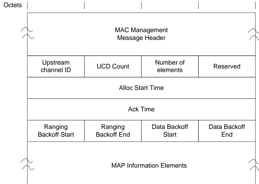
Figure 6–18 - MAP Format
