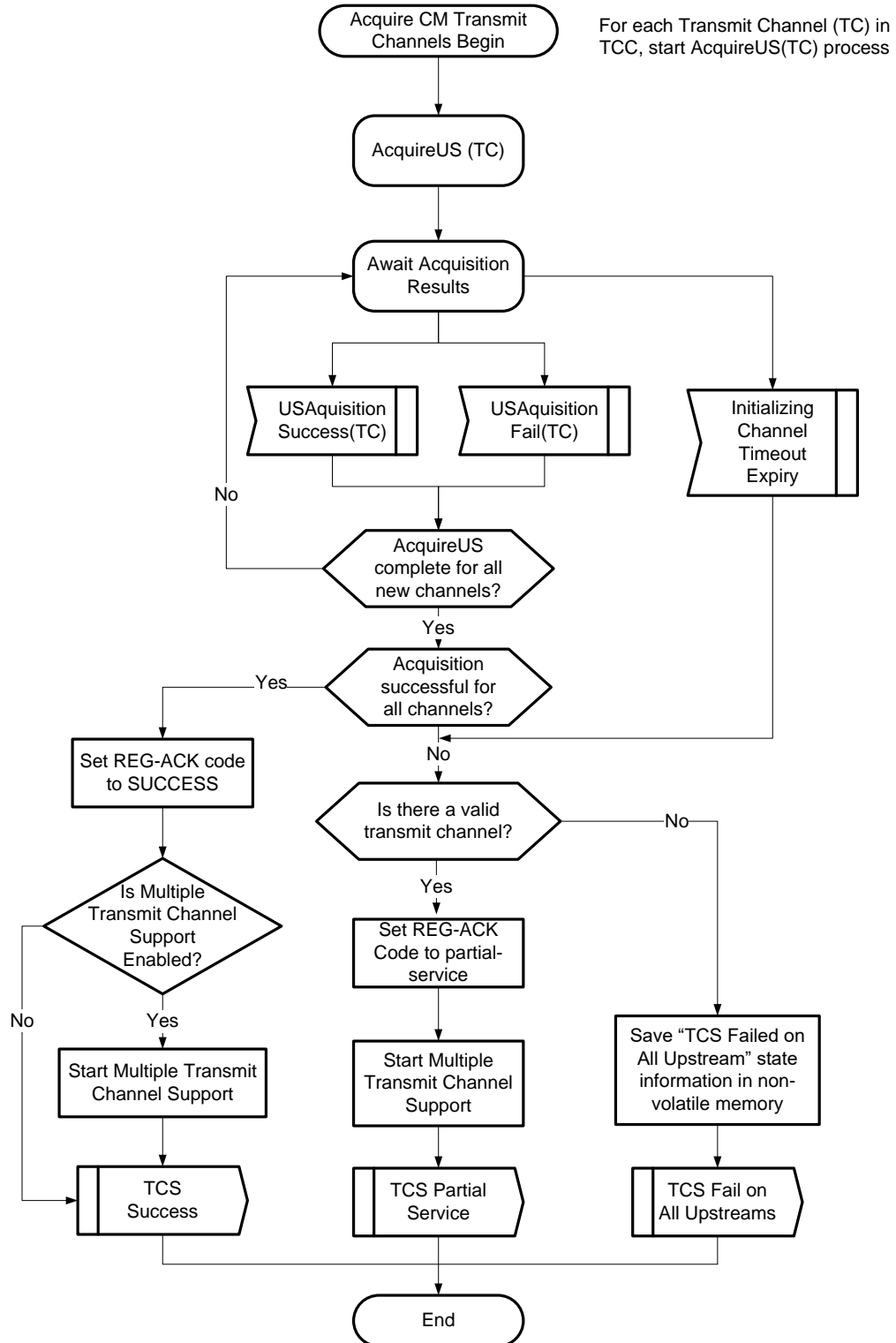
Figure 10-28 - CM Acquires Transmit Channels
