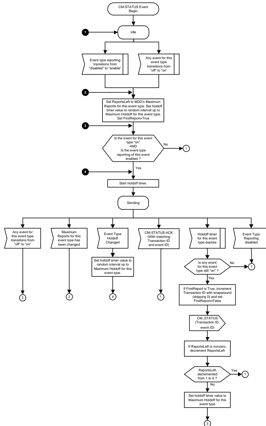
Figure 10-36 - CM-STATUS Event Type State Machine
