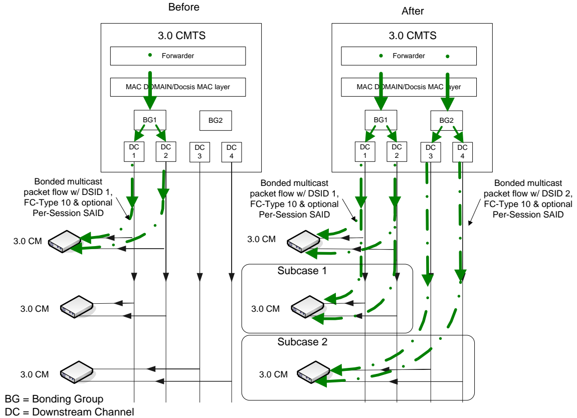
Figure VIII-8 - Multicast session replication to clients behind two 3.0 CMTS
