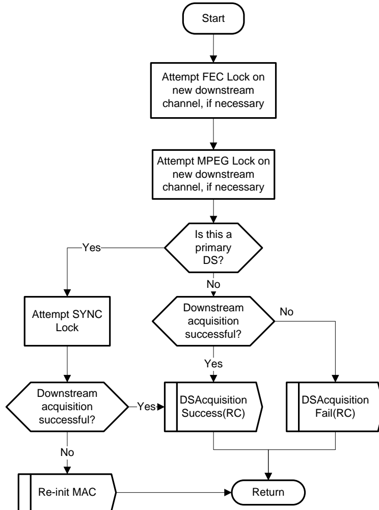
Figure 11-57 - CM AcquireDS Procedure
