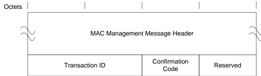
Figure 6–40 - Dynamic Service Deletion — Response
