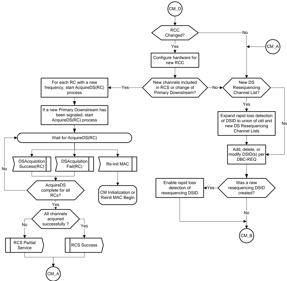
Figure 11-55 - CM DBC-RSP (part 2)
