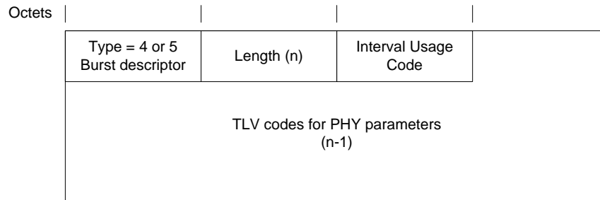
Figure 6–16 - Top-Level Encoding for Burst Descriptors
