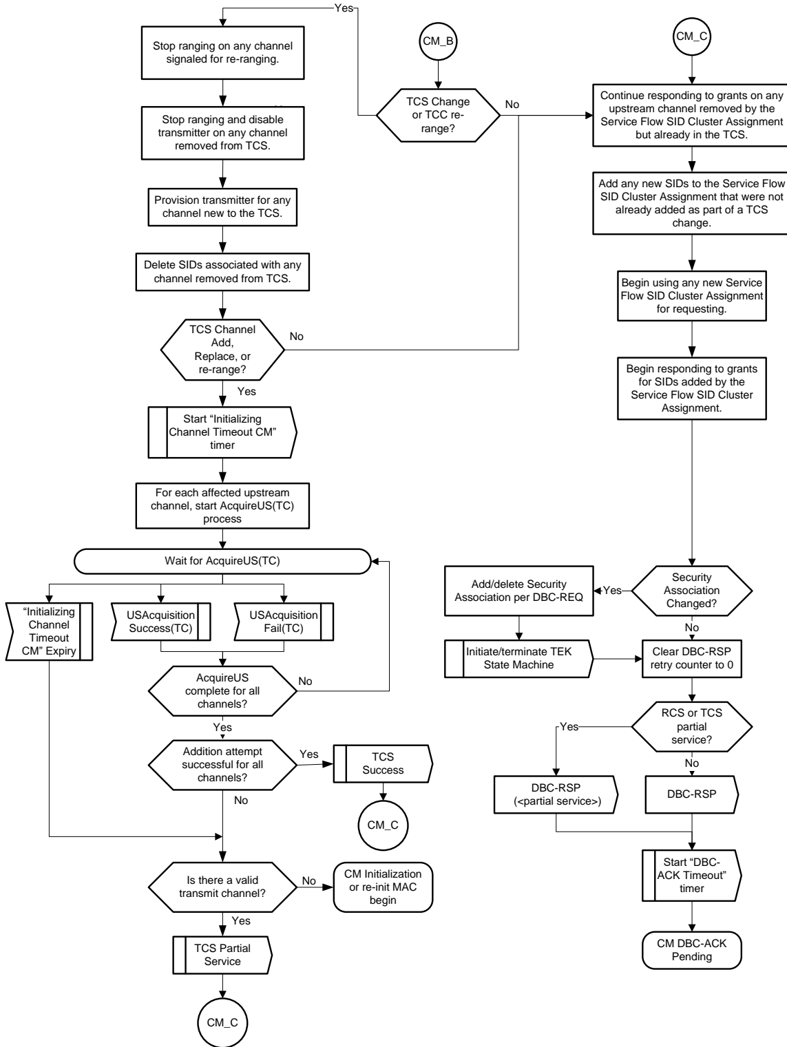
Figure 11-56 - CM DBC-RSP (part 3)
