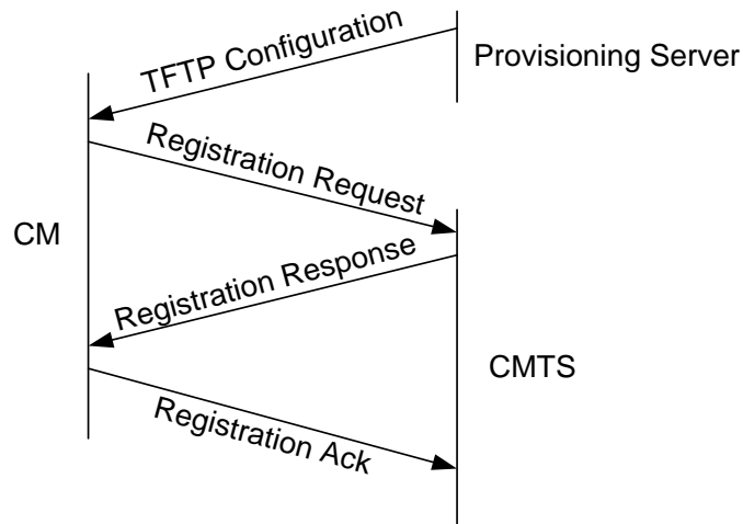
Figure 7-14 - Registration Message Flow
