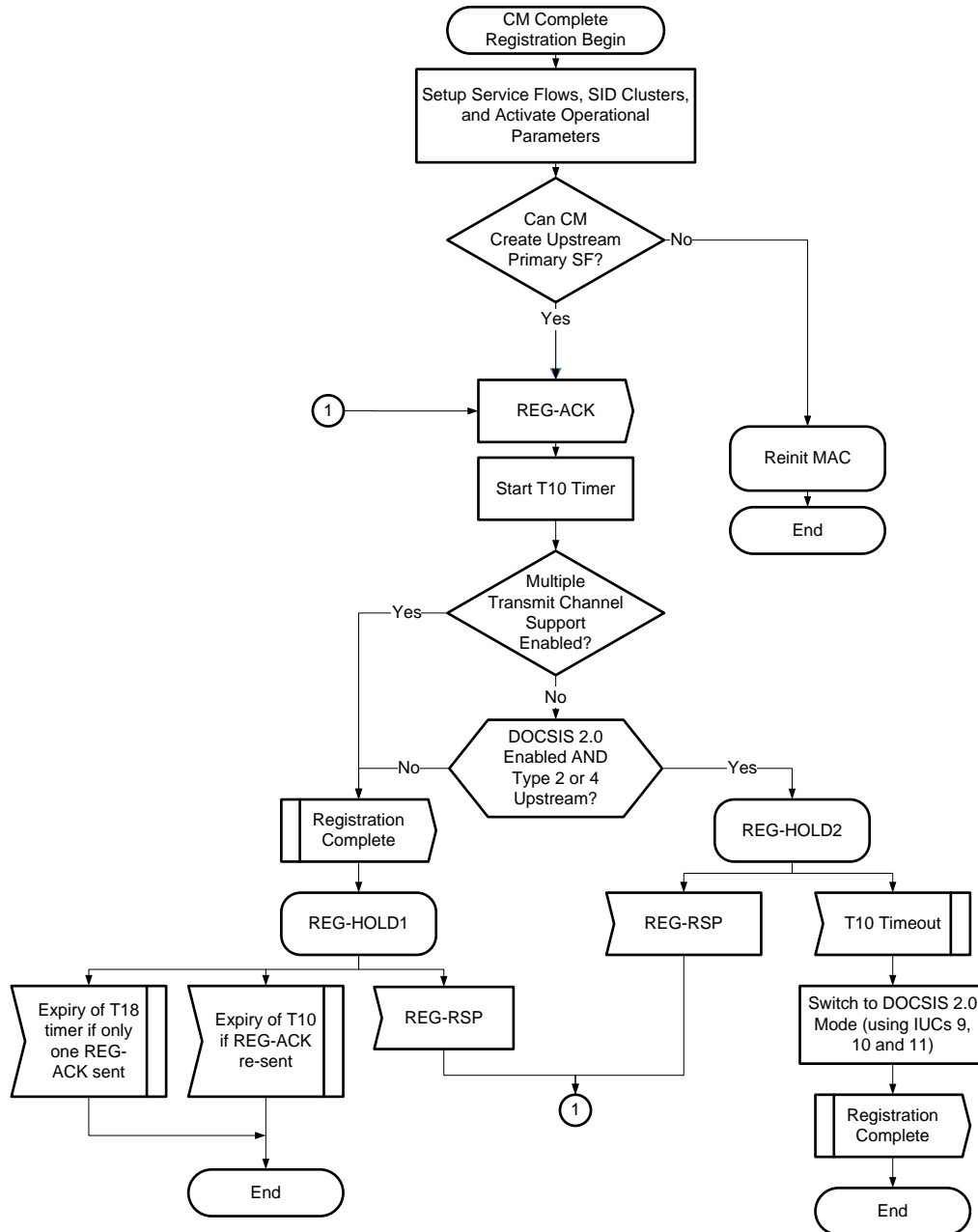
Figure 10–30 - CM Completes Registration
