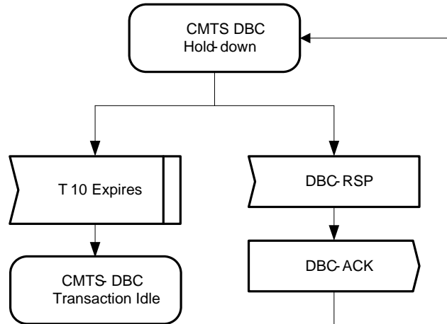
Figure 11-53 - CMTS DBC Hold-down
