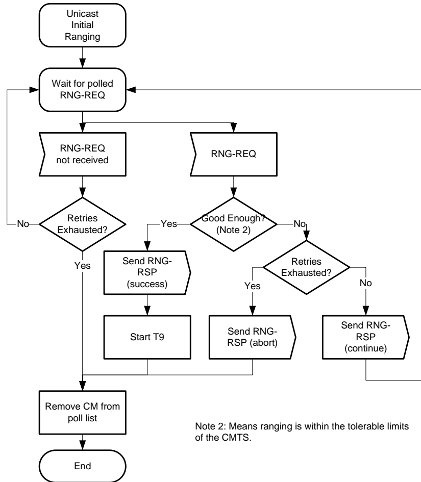
Figure 10-15 - Unicast Initial Ranging – CMTS
