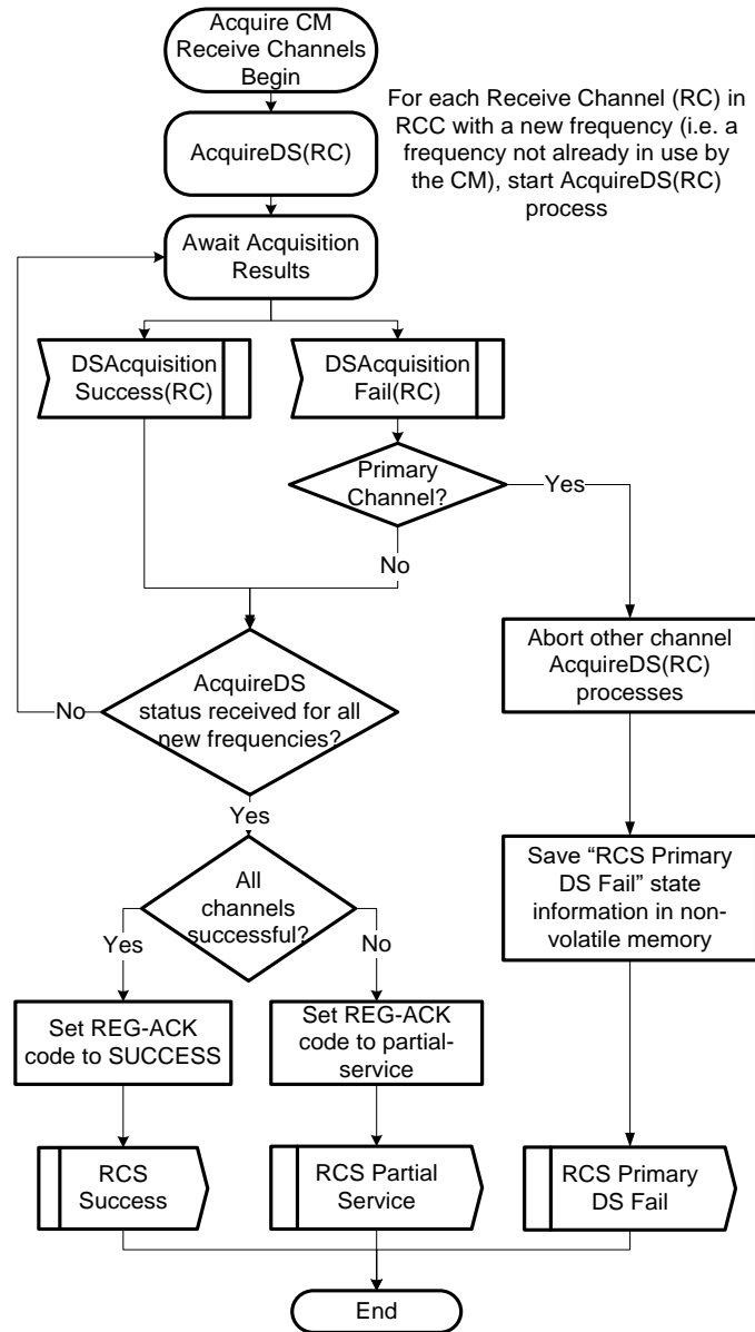
Figure 10–26 - CM Acquires Receive Channels
