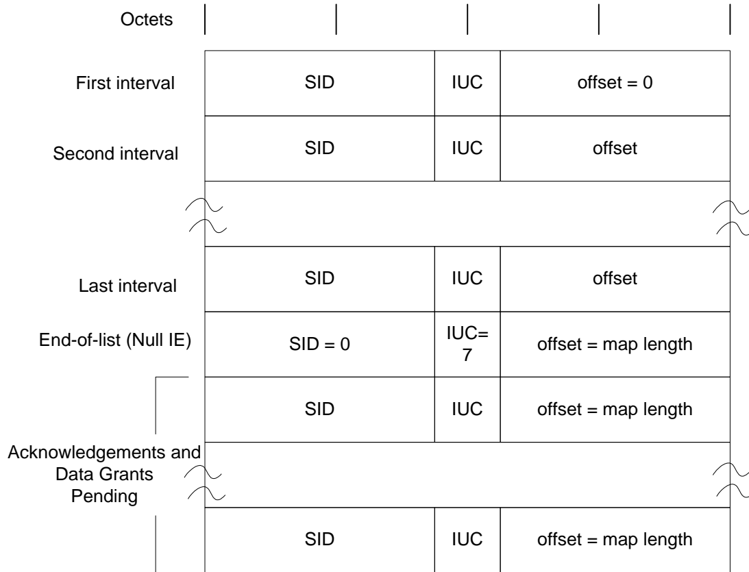
Figure 6–19 - MAP Information Element Structure
