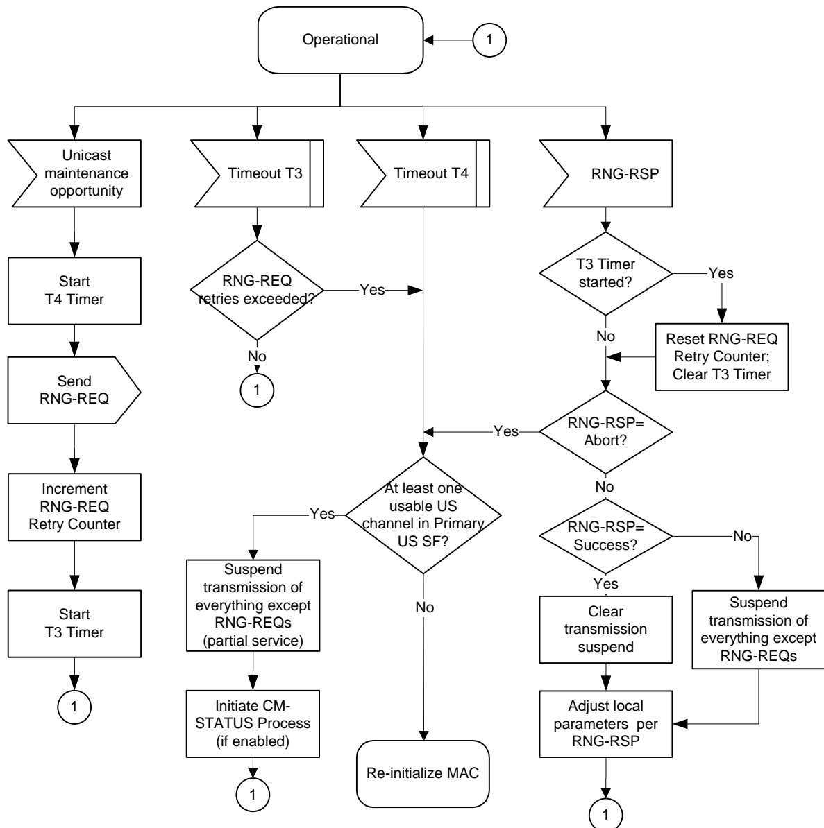
Figure 10-35 - Periodic Ranging - CM View
