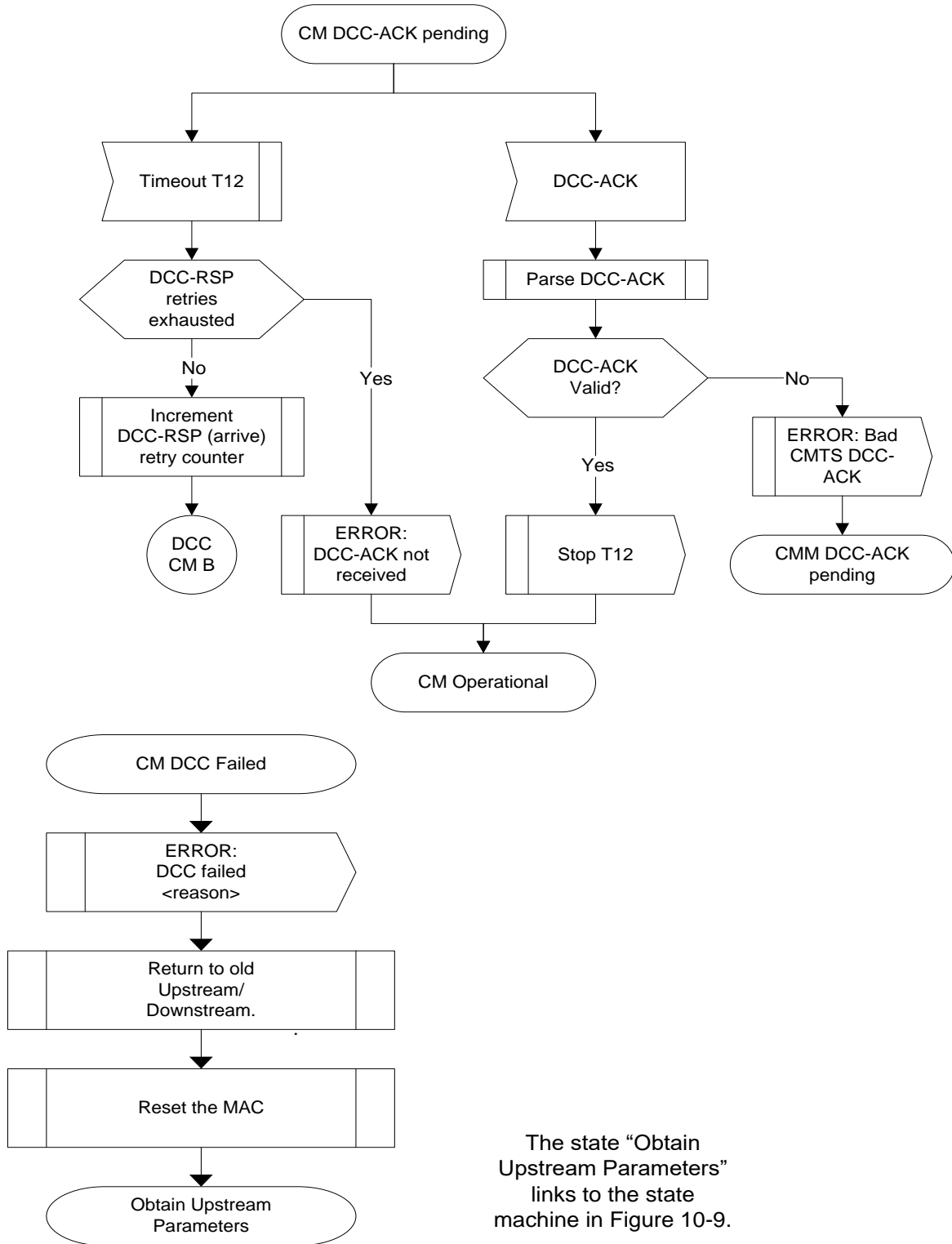
Figure 11-49 - Dynamically Changing Channels: CM View Part 4
