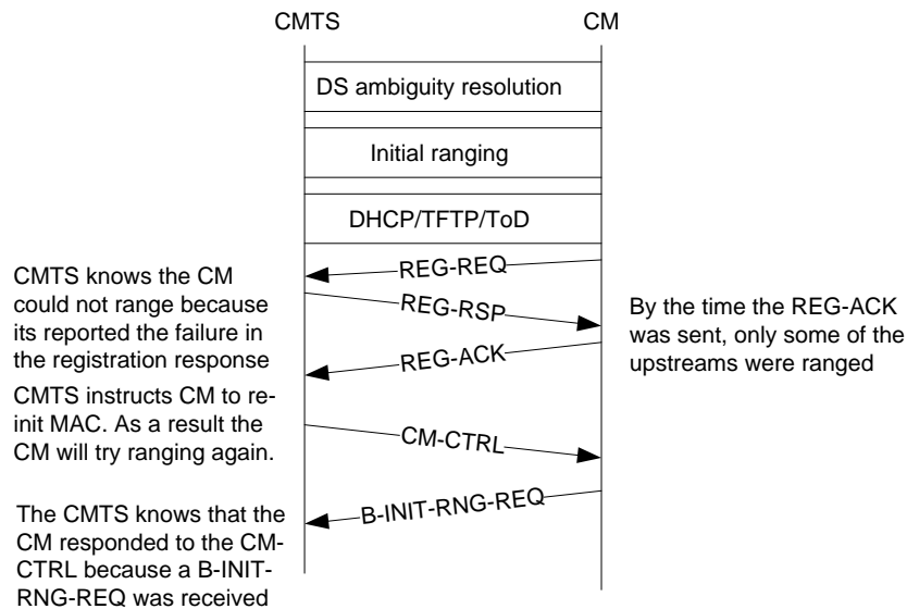
Figure V-1 - Example 1 - Modem can't range on all upstreams
