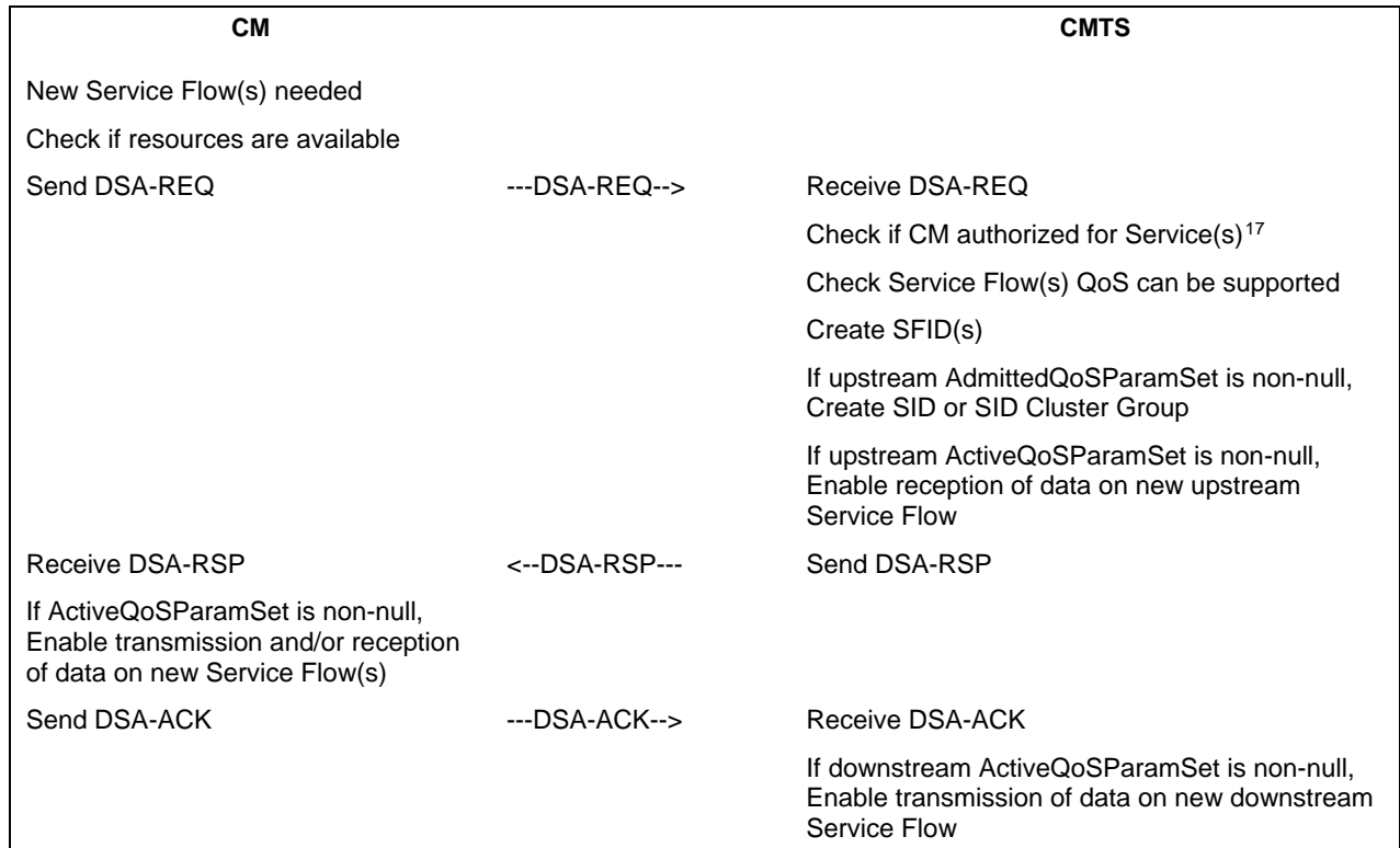
Figure 11–9 - Dynamic Service Addition Initiated from CM
