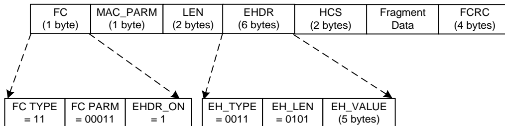
Figure 6-8 - Fragmentation MAC Header Format
