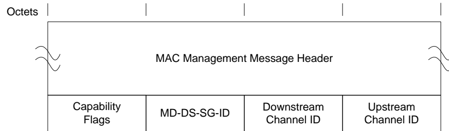
Figure 6–22 - B-INIT-RNG-REQ Format 6
