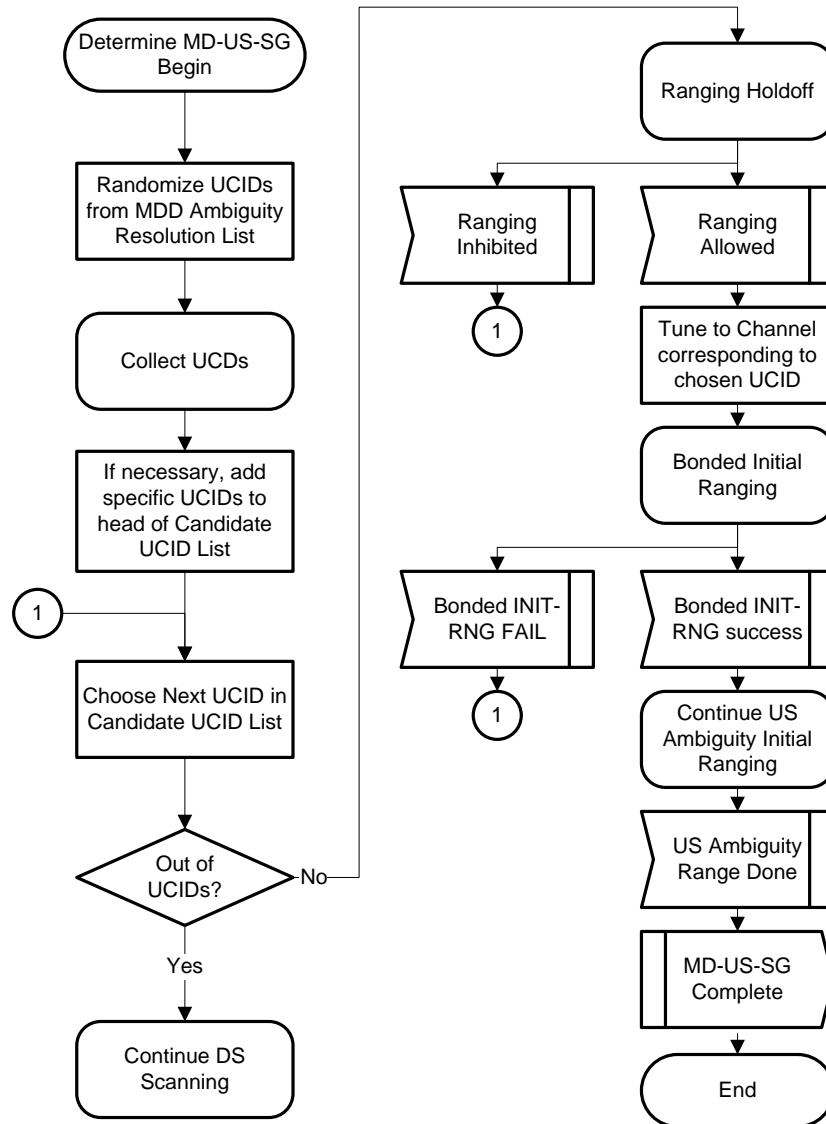
Figure 10–6 - Determine MD-US-SG
