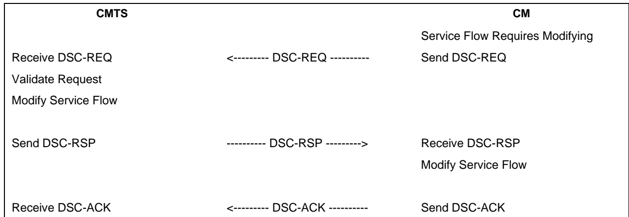
Figure 11–20 - CM-Initiated DSC
