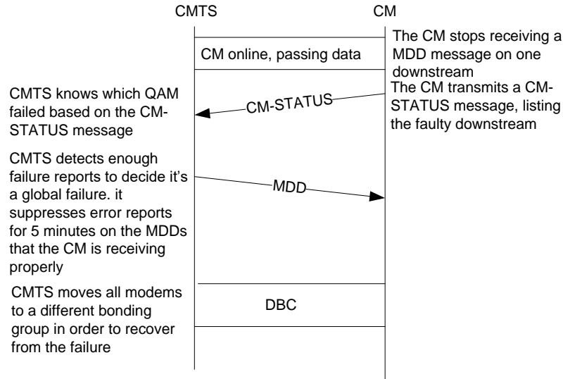
Figure V-2 - Example 2 - Option 4 20
