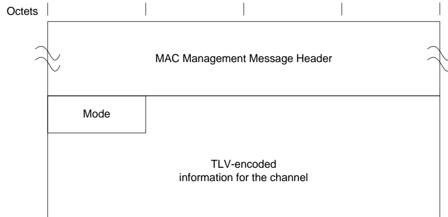
Figure 6–47 - Test Request
