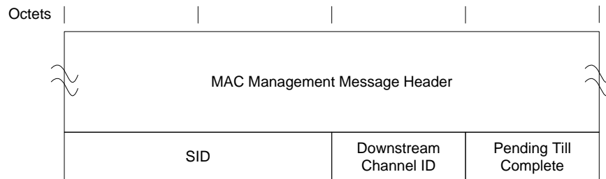
Figure 6–20 - RNG-REQ Format
