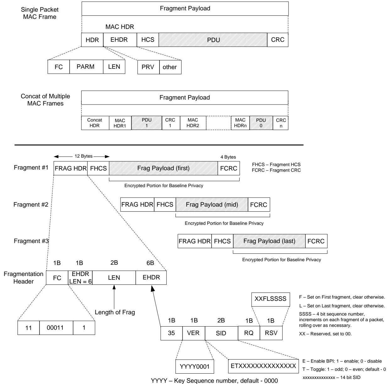
Figure 7-6 - Fragmentation Details
