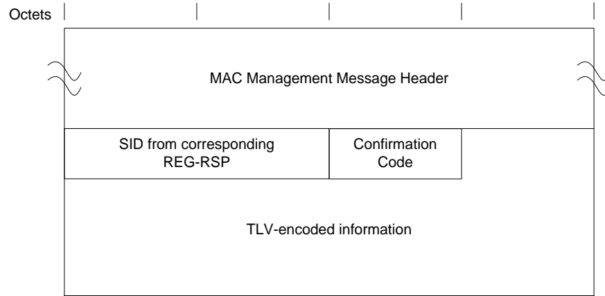
Figure 6–30 - Registration Acknowledgment
