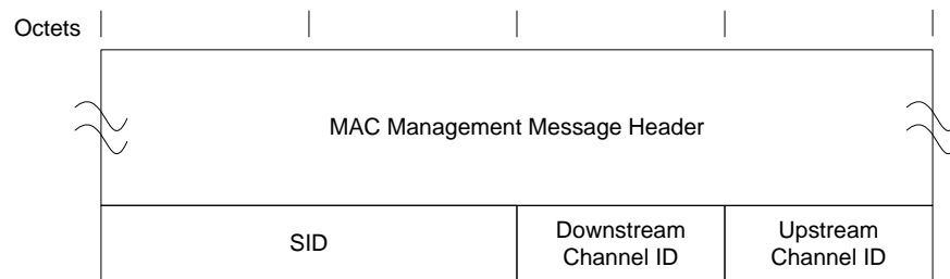
Figure 6–21 - INIT-RNG-REQ Format
