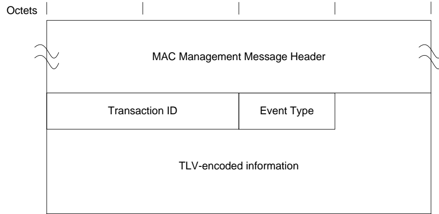
Figure 6-54 - CM-STATUS Report
