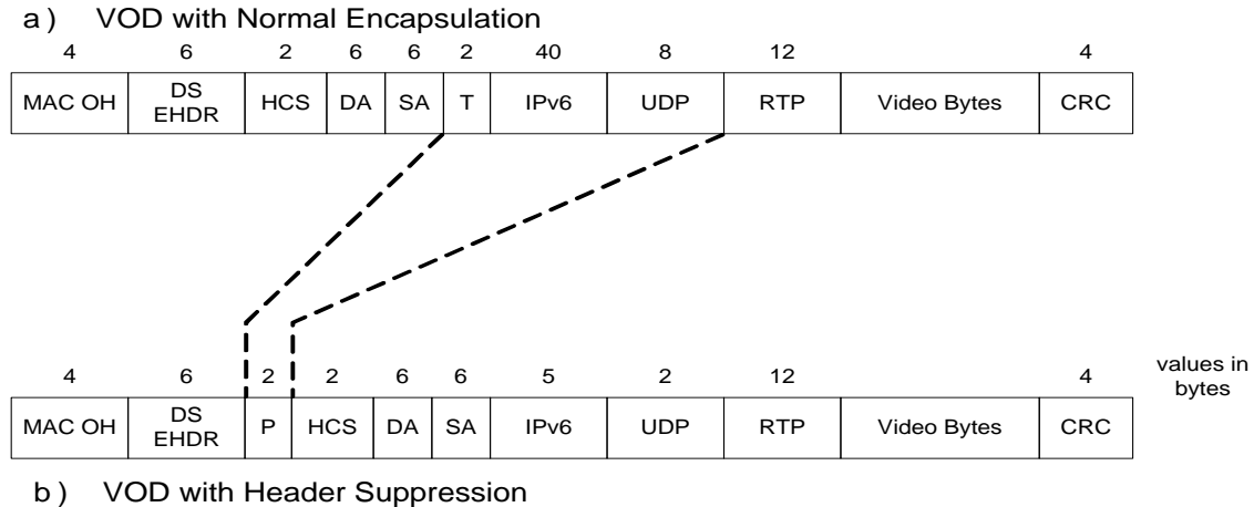
Figure 7-24 - DSID-Indexed Payload Header Suppression Example
